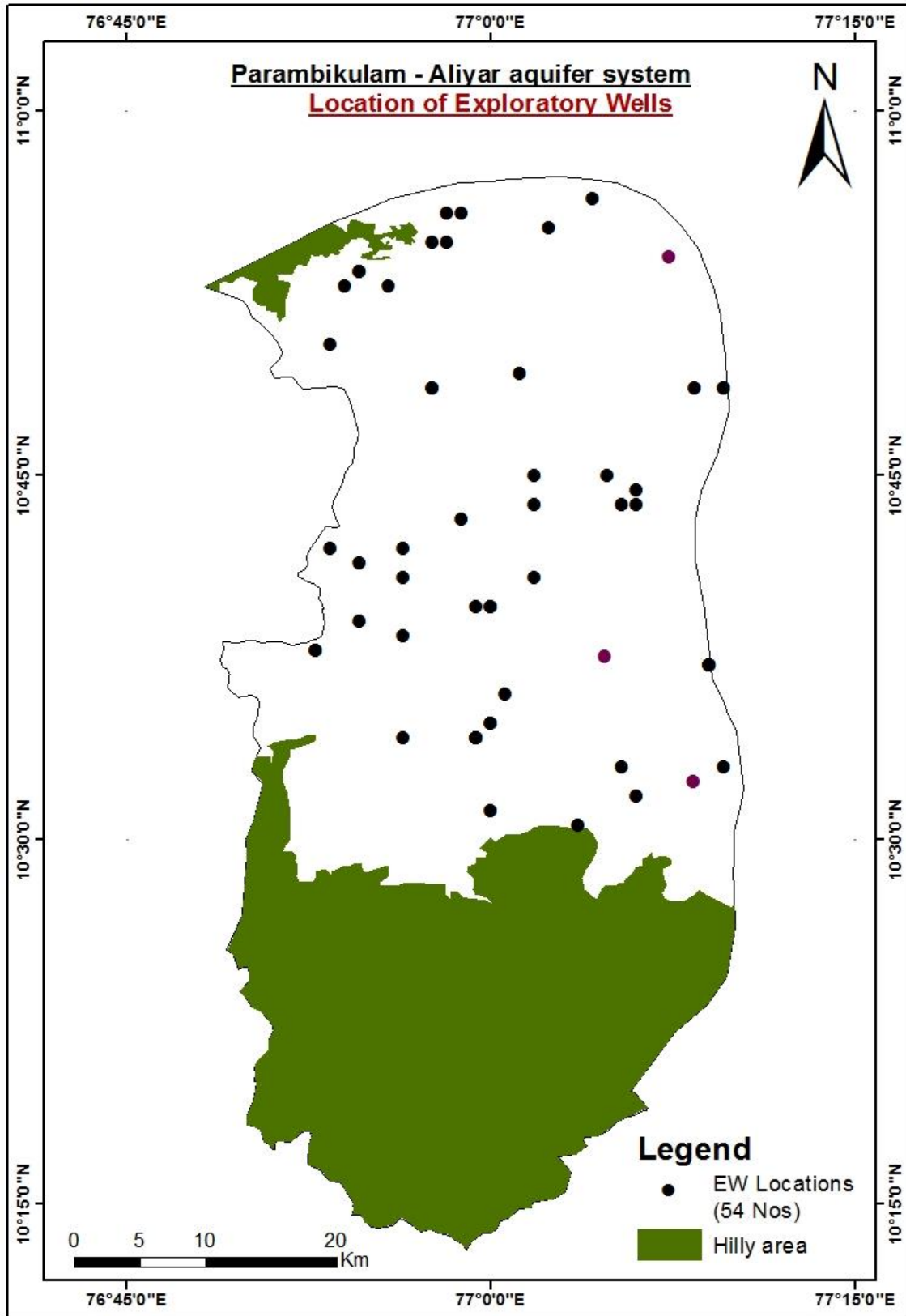
Figure 3.1. Locations of Exploratory Wells
