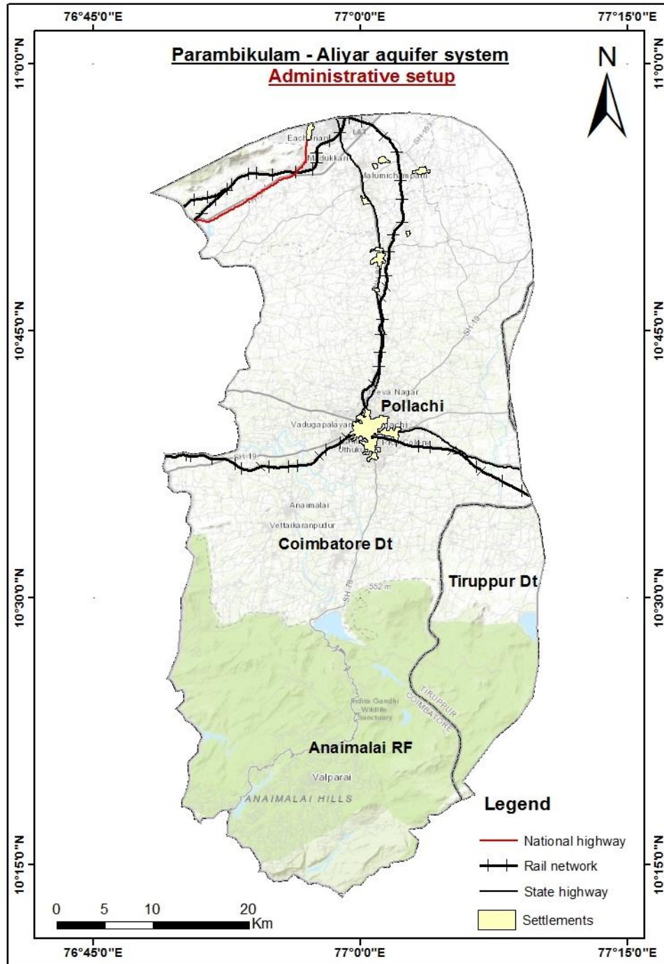
Figure 1.2a. Administrative setup and connectivity of the Parambikulam – Aliyar Aquifer System
