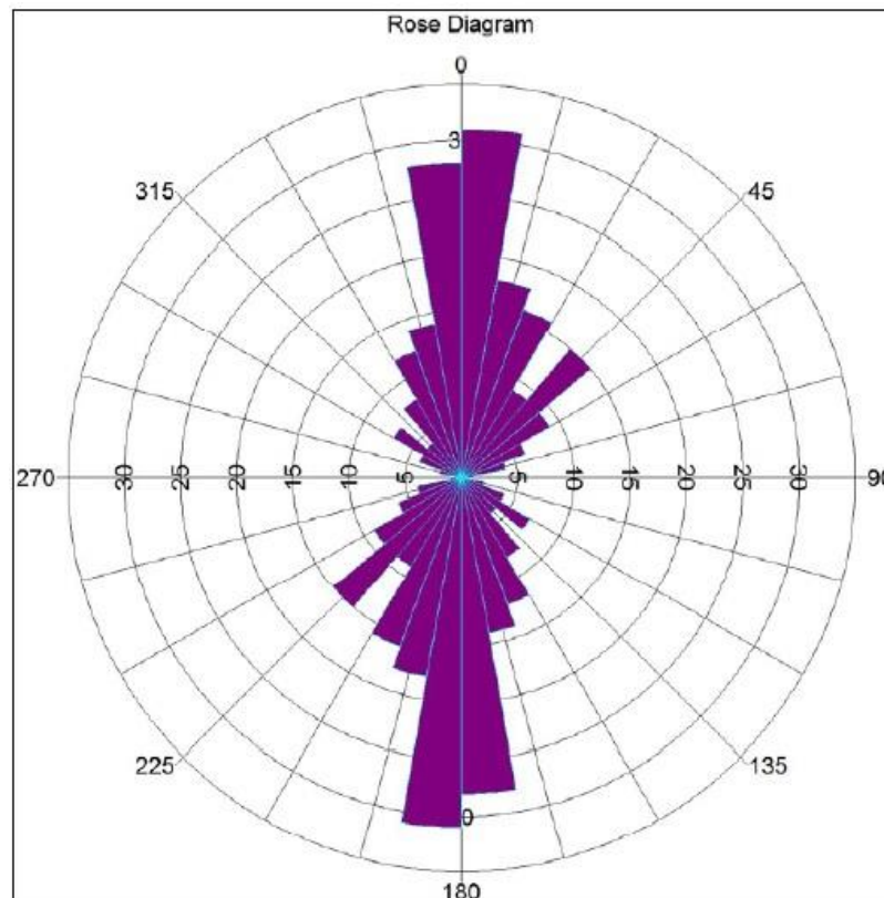
Figure 4.1: Rose Diagram showing orientation of lineaments
